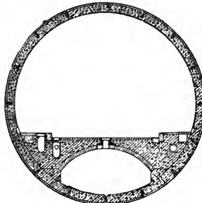
Rotherhithe, Thames. 1 tube
