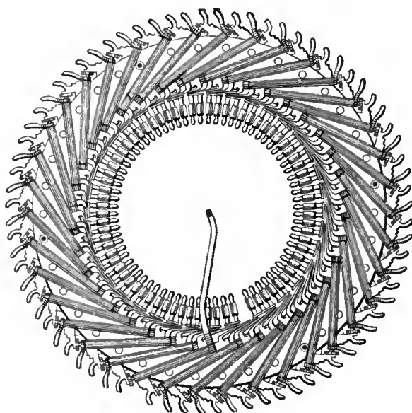
FIG. 4.—Type-bar Bearings, Smith Premier.
