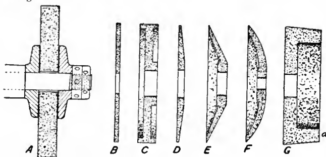
FIG. 53.—Typical Grinding Wheels.
