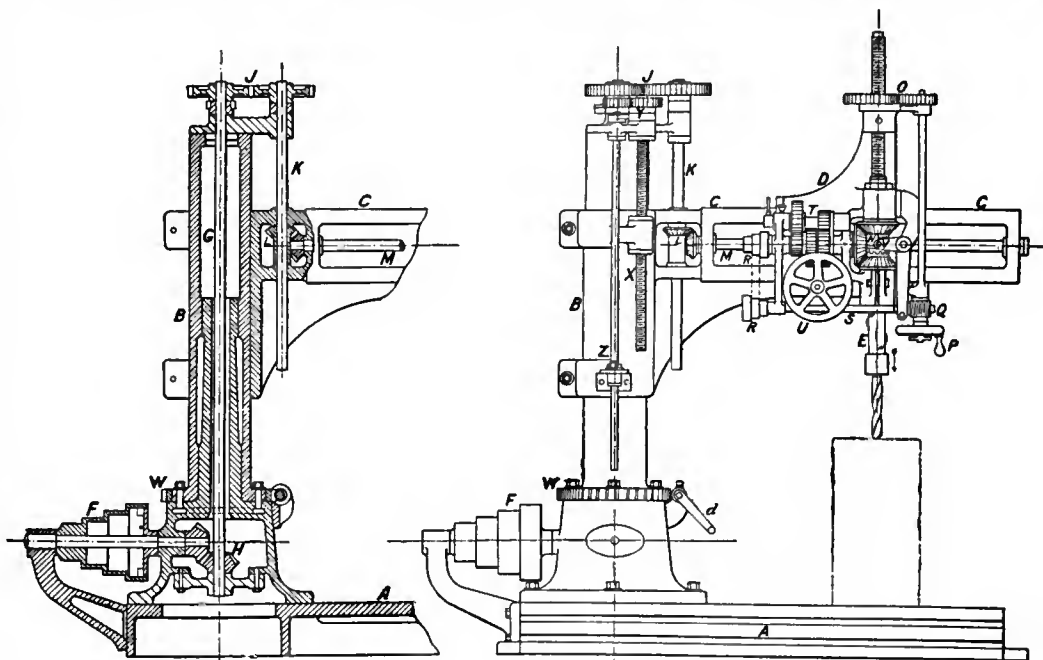
FIG. 46.—Pillar Radial Drilling Machine, 5 ft. radius.
