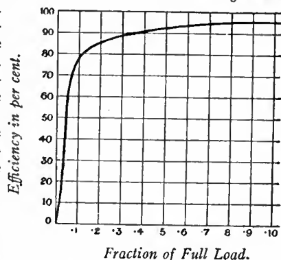
FIG. 4.—Typical Efficiency Curve of Closed Circuit Transformer.
