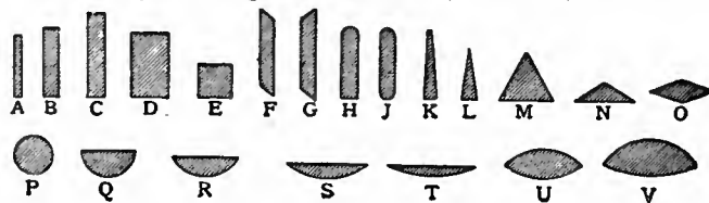
FIG. 22.—Cross-sectional Shapes of Files.
