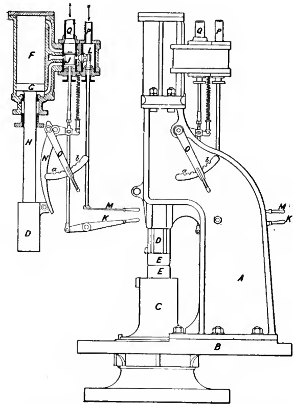
FIG. 57.—Steam Hammer, small Overhanging Type. (B. & S. Massey, Manchester).
