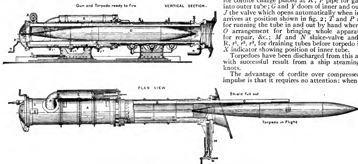
FIG. 3.—Broadside Submerged 18-in. Torpedo Tube.
