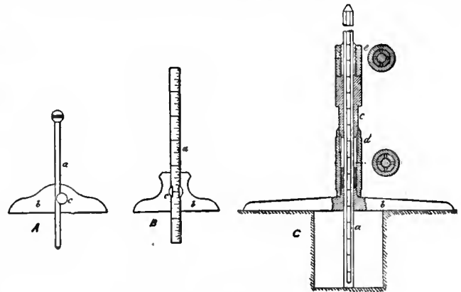
FIG. 74.—Depth Gauges.
