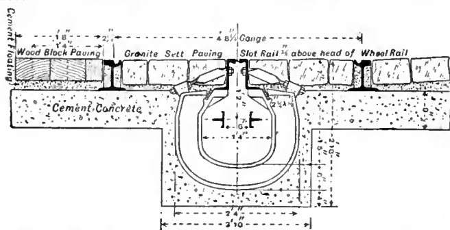
FIG. 8.—Cross-section of Open Conduit Road (American type).
