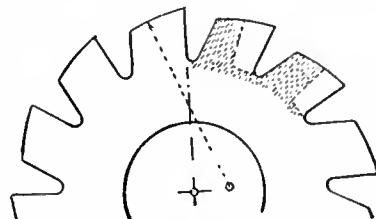
FIG. 20.—Relieved Teeth of Milling Cutter.
