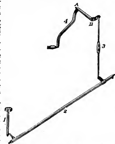
FIG. 5.—Rocking-shaft Mechanism of Smith Premier.
