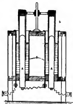
FIG. 12.—Section through Nodon Valve.
