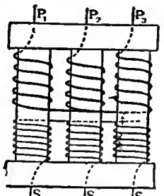
FIG. 8.—Brush Three-phase Transformer.
