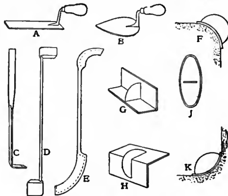
FIG. 28.—Moulding Tools.
