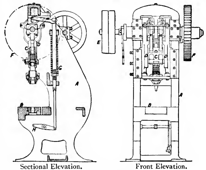
FIG. 62.—Power Press.
