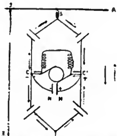
FIG. 13.—Method of connecting the cells.
