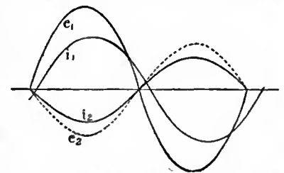
FIG. 7.—Transformer Curves at full load.
