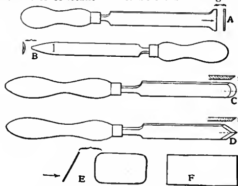
FIG. 21.—Group of Scrapers.
