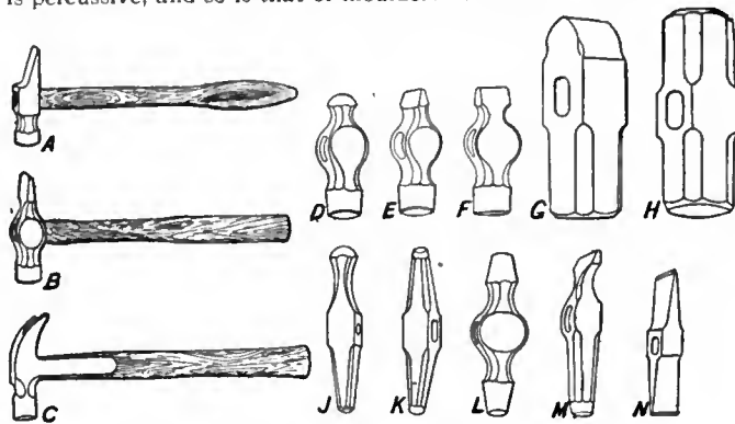
FIG. 27.—Hammers.
