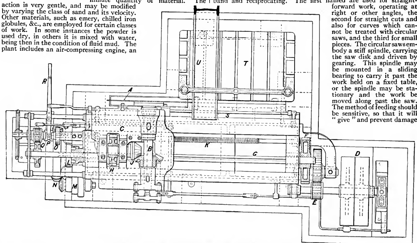
FIG. 55.—Cold-sawing Machine. (Isaac Hill & Son, Derby.)
