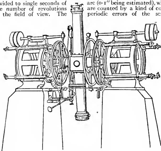
Transit Circle.
