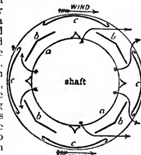
FIG. 4.—Sectional Plan of Buchan's Exhaust Cowl.
