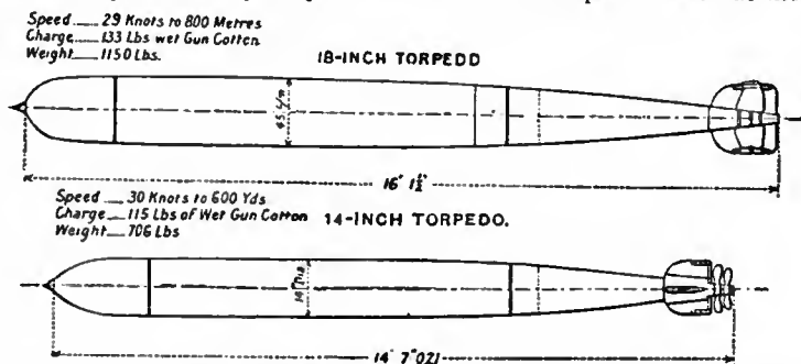
FIG. 1.—Diagrams of 14- and 18-in. Torpedoes.
