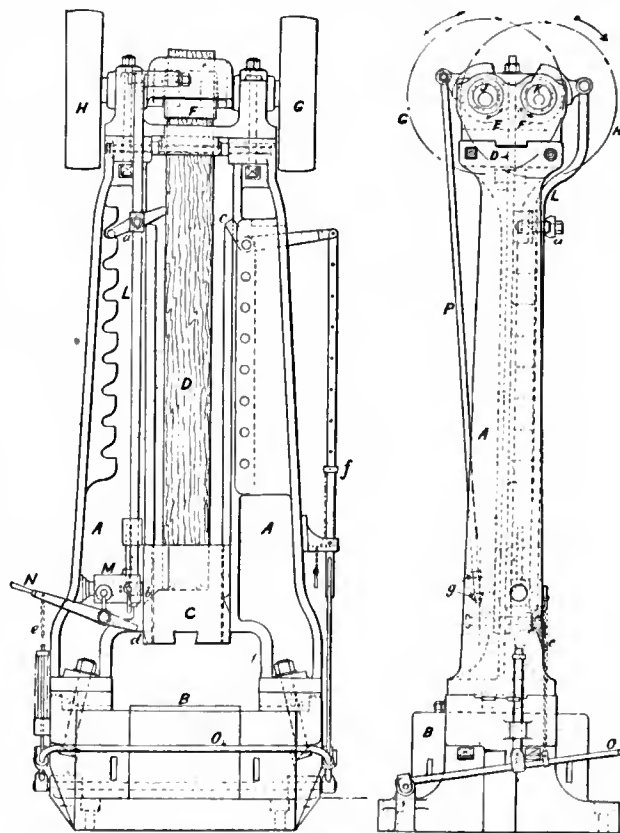
FIG. 59.—Drop Hammer—board type. (B. & S. Massey, Manchester.)
